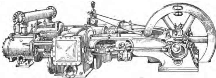
FIG. 55.—Duplex cross compound steam, two-stage air compressor.
